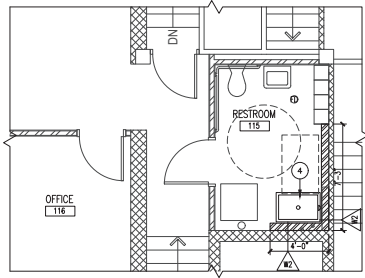
← 2 FLOOR PLAN - RESTROOM SCALE: 1/4" = 1'-0"
