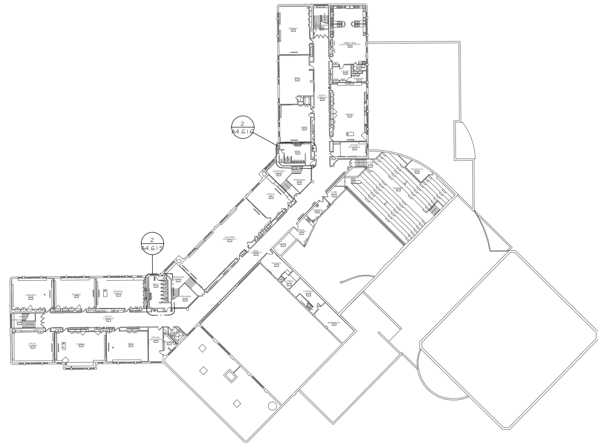
3 Callanan Second Floor 1/32" = 1'-0"
